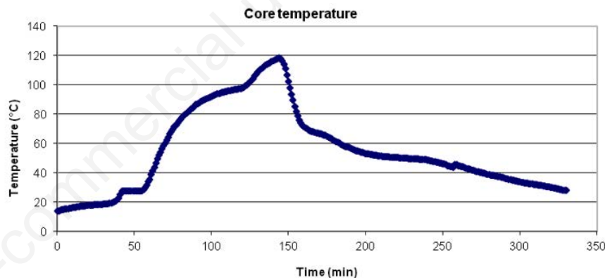
Figure 2. Most unfavourable thermal profile logged during the thermal treatment.
